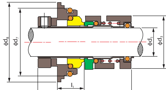
TS CR-22, Punched TYPE
