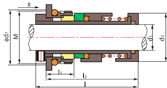
TS CR-12,14,16 Machined TYPE
