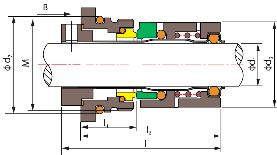
TS CR-12,14,16 Punched TYPE
