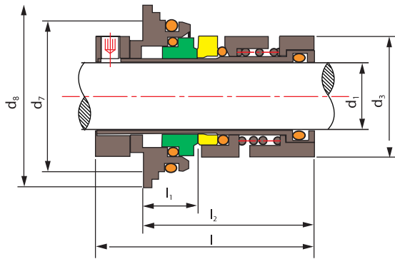
TS CR-22,32 Machined TYPE
